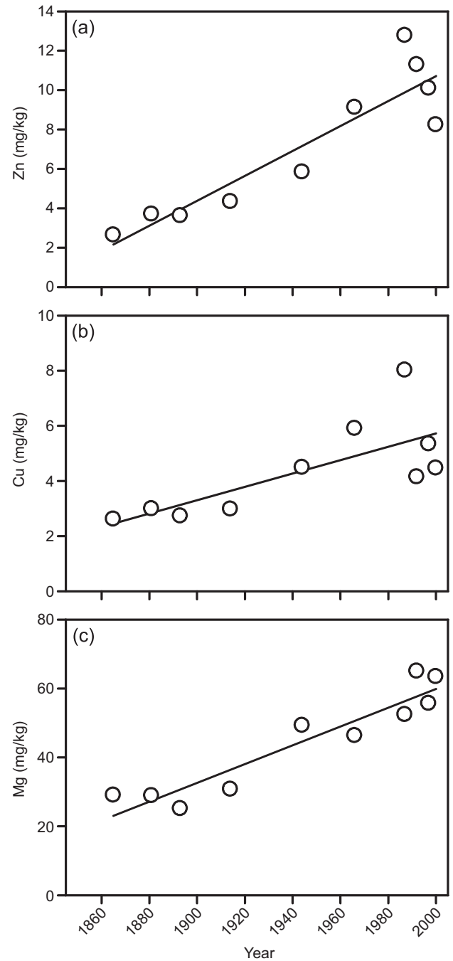
Fig. 4. Changes in the EDTA-extractable concentrations of Zn (a) and Cu (b) and ammonium nitrate-extractable Mg (c) in the soils from the N_2PKNaMgS plot.
