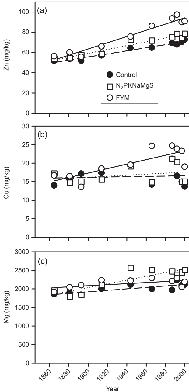
Fig. 3. Changes in the total concentrations of Zn (a), Cu (b) and Mg (c) in the soils from three plots of the Broadbalk Experiment. Lines represent regression lines: dashed line for the control, dotted line for N_2PKNaMgS , and solid line for FYM.
