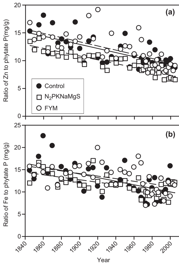
Fig. 2. The ratio of Zn (a) or Fe (b) to phytate P in wheat grain from three plots of the Broadbalk Experiment since 1845. Lines represent regression lines: dashed line for the control, dotted line for N_2PKNaMgS , and solid line for FYM.
